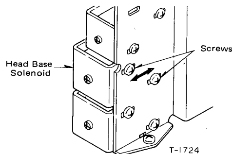
Fig. 4-3 Head base solenoid location
