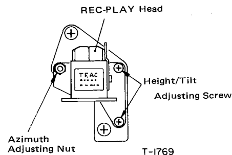
Fig. 5-3 Azimuth adj. nut location
