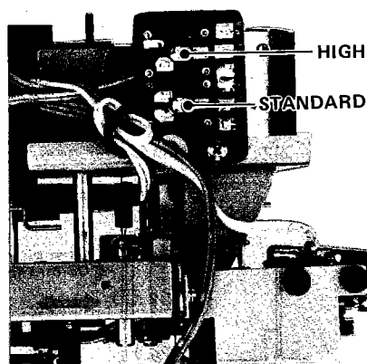
Fig. 4-6 Tape speed adjustment location
