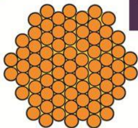
IMAGE DRAWING of Gold & Silver micro particles dispersed Colloidal Liquid soaked on the Surface of 72-Strings of 0.32mm \phi PC-Triple C Conductors *[micro particles diameter is about 3.5~8mm/ 1,000,000]
