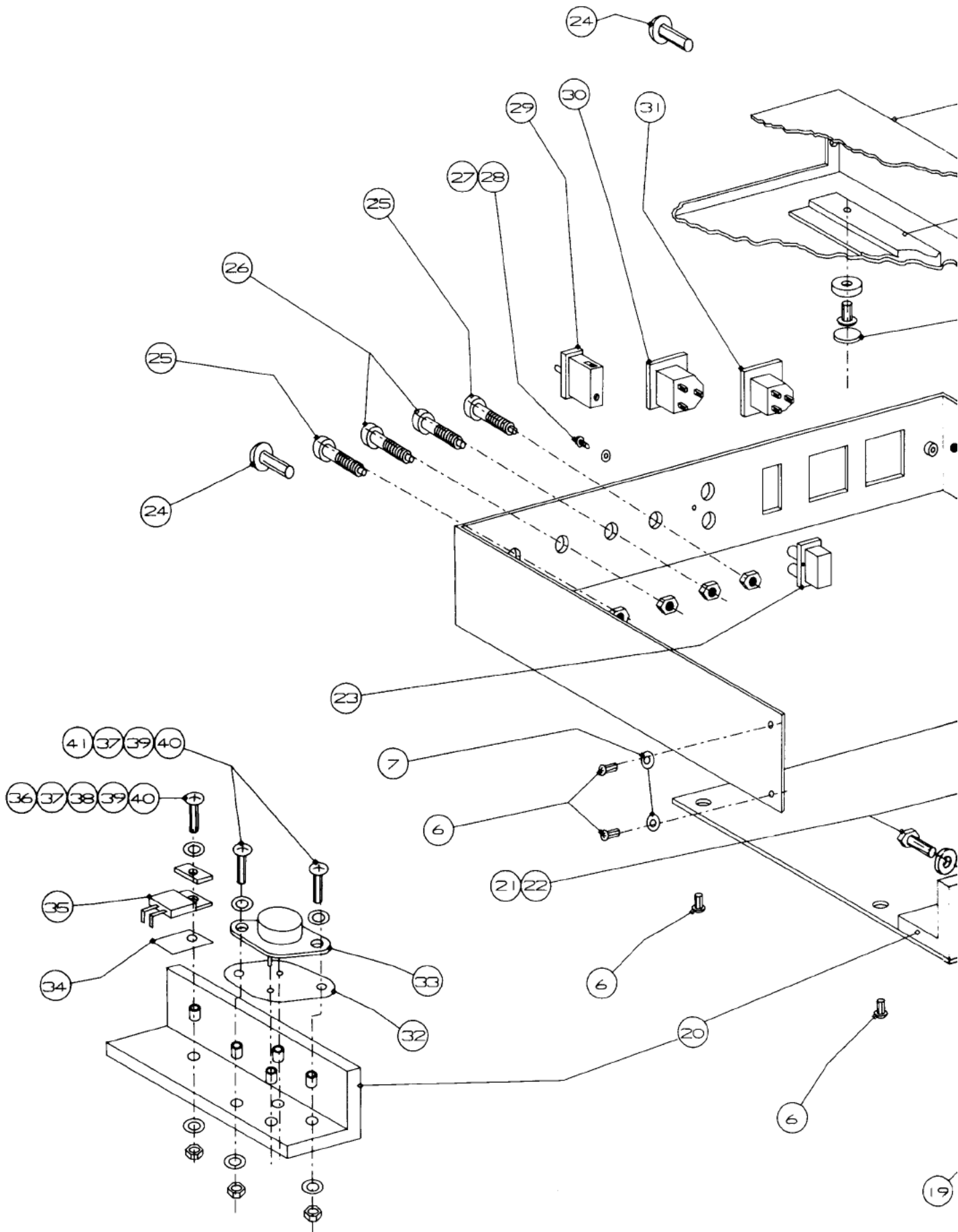
Fig 1 Exploded View
