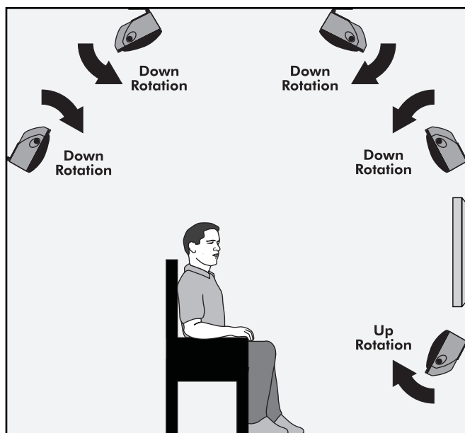
Figure 4. Horizontal Installation. Rotation direction for various installation locations.
